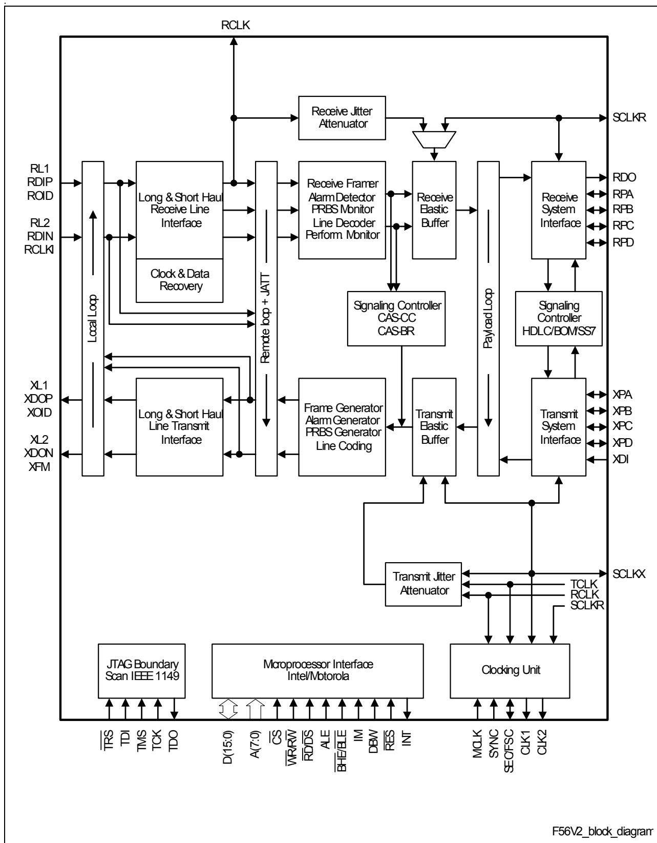
Figure 5 Block Diagram
